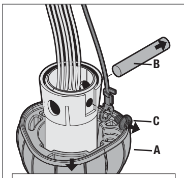
Slide ball down (A), remove small metal pin (B) and ground screw and grounding wire (C).
