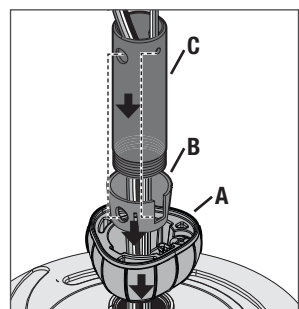
Route wiring harnesses from the fan through the accessory downrod (C). Slide inner sleeve (B) and ball (A) over downrod. Make sure to align the holes for the sleeve (B) and downrod (C).
